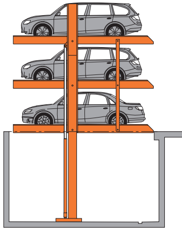
System lifted
